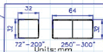
Frame section
