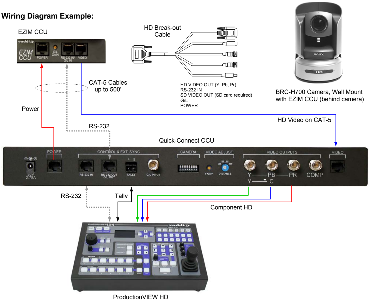
Figure 2: The Quick-Connect CCU System uses a Cat. 5 (all 4-pairs) for power to ensure the motors receive the required current to operate properly. The Video Cat. 5 cable uses all four pairs for video. The RS-232 Cat. 5 provides communication to the camera for CCU and PTZ control and G/L (where applicable) to the camera. These Cat. 5 cables can be run up to 500' (152.4m). See Appendix 1 for wiring and pin-out information. NOTE: A direct RS-232 Cat. 5 cable is required for each Quick-Connect CCU and camera. Daisy-Chain configurations are not supported.
