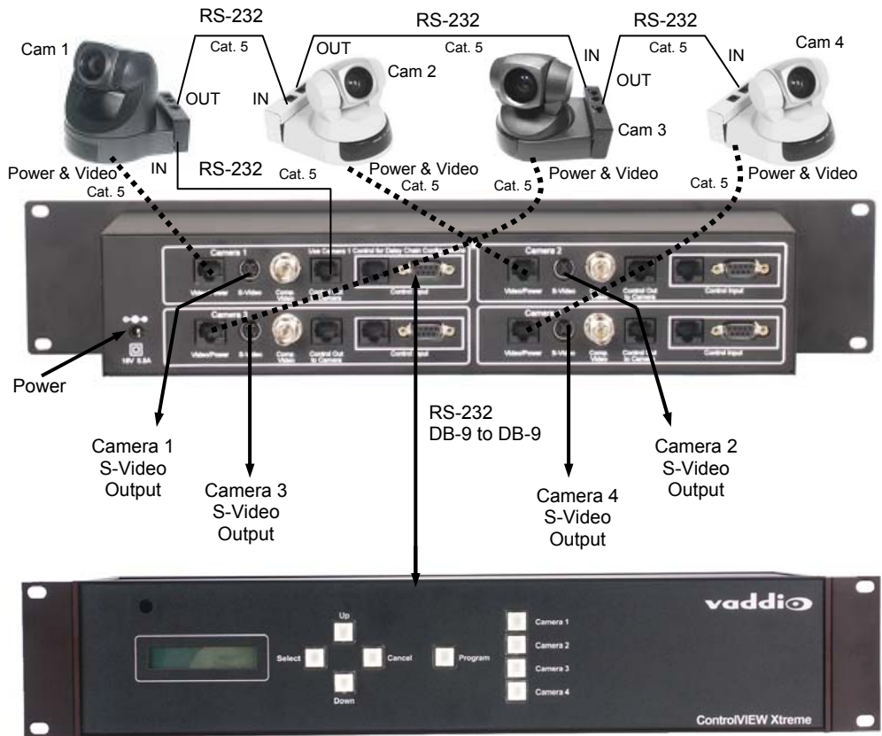
Figure 4: Daisy Chain Example with Single Control Port
